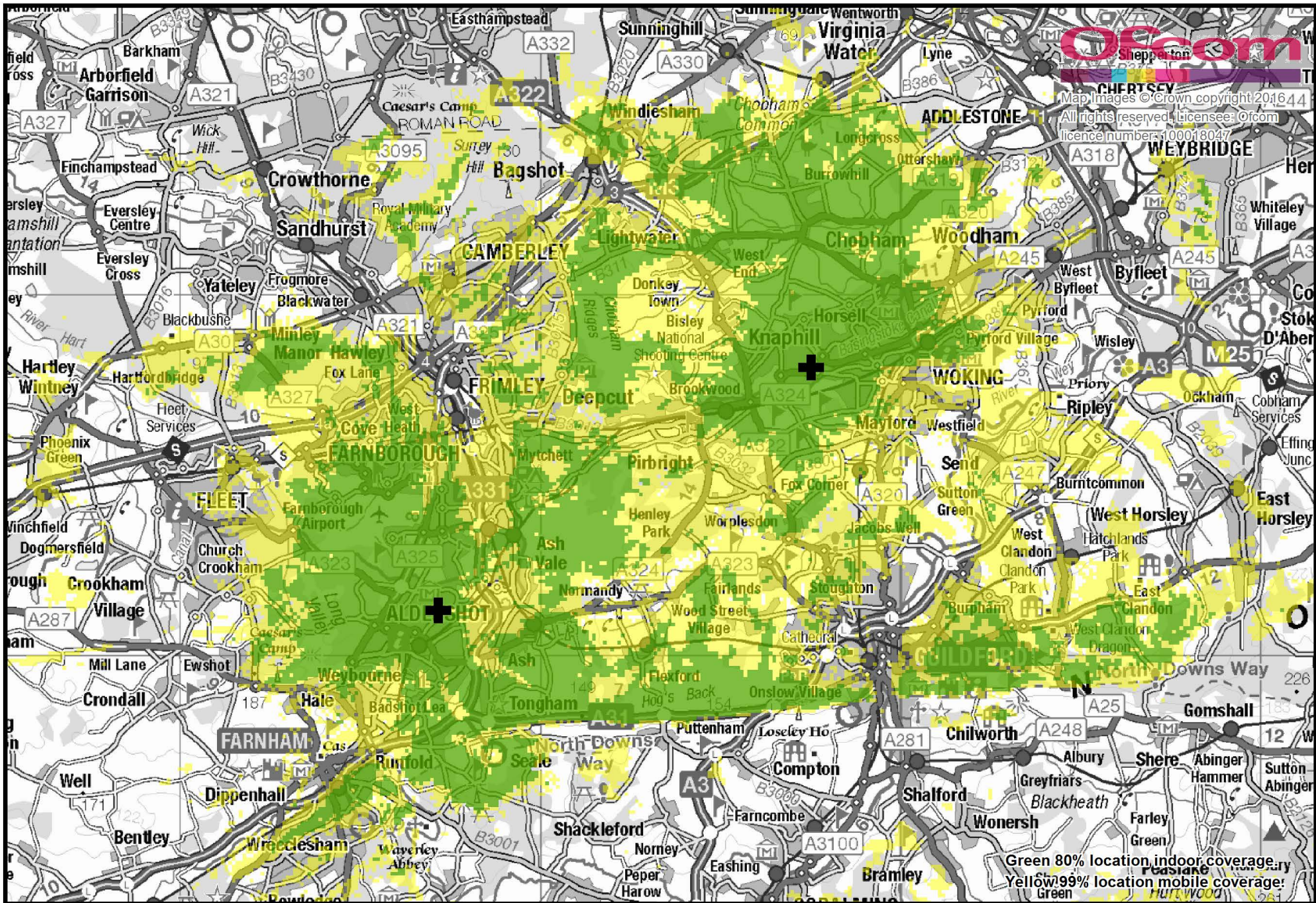
Woking & Aldershot small scale DAB trial predicted coverage. November 2016.
